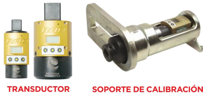
TRANSDUCTOR
